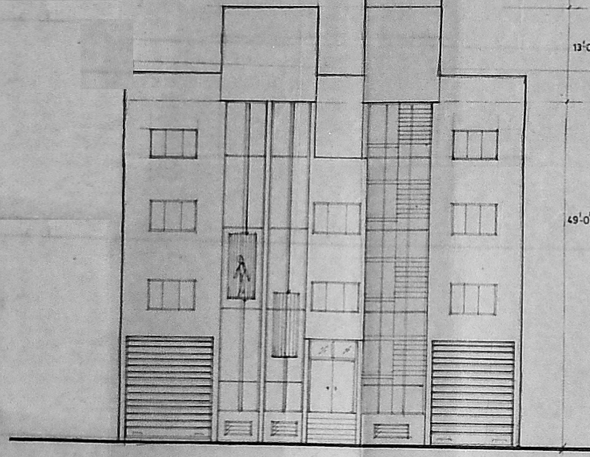
FRONT ELEVATION
